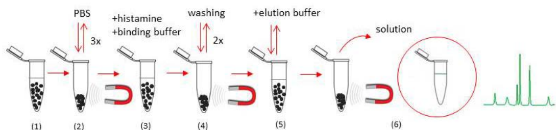
Figure 1 Experimental workflow
